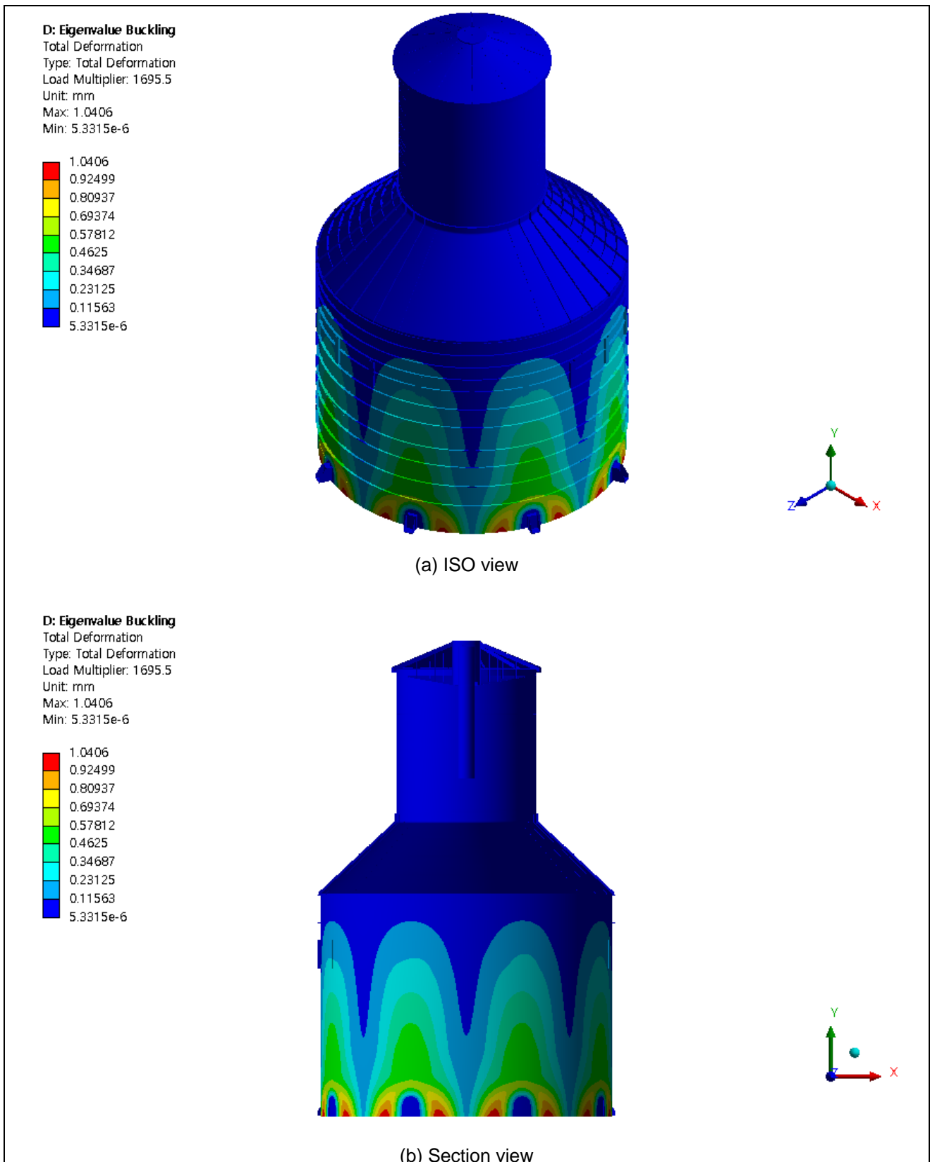
Fig. 6.6 Linear buckling
